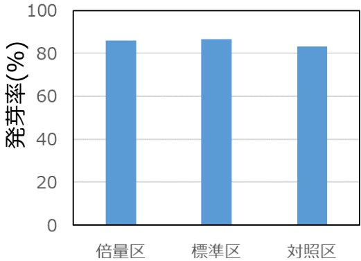
発芽率 (6/2播種)
