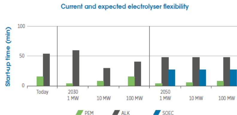
Figure 5: Start-up times for electrolyzers
